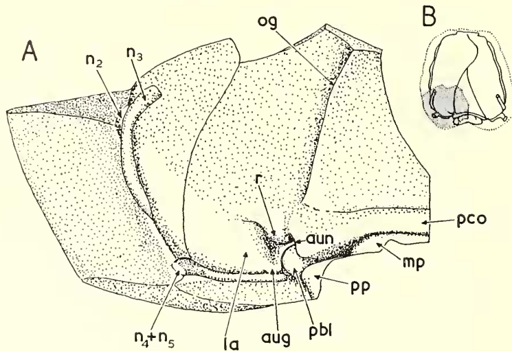
TEXT-FIG. 15. A, Portion of internal mould of Mitrocystites mitra to show auditory nerve and ganglion (MCZ 566, cf. Pl. 98, fig. 7). B, Diagram of dorsal aspect of theca, to show portion (stippled) included in A. aug = auditory ganglion; aun = auditory nerve; la = left atrium; mp = medial part of brain; n_2 , n_3 , n_{4+5} = nerves of left palmar complex; og = oblique groove; pco = posterior coelom; pp = posterior part of brain; r = rectum. For meaning of anatomical terms see Jefferies 1967, p. 179ff.; 1968, p. 315ff.
